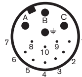
Abb. 1: Servomotor: Connector, 14-pole (male; view to servomotor)
