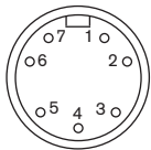
Abb. 2: Servomotor: Connector, 7-pole (female; view to servomotor)
