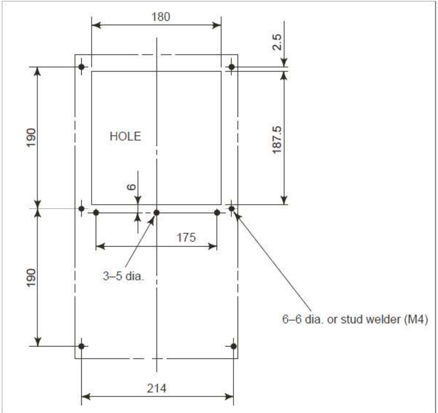
Heat Pipe Type Heat Exchanger (CE Mark) - Panel Cut
