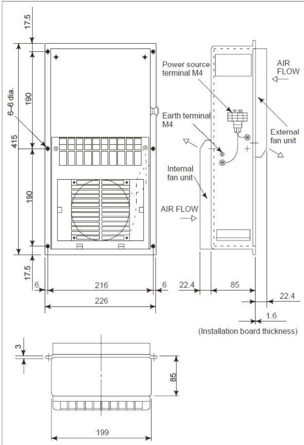
Heat Pipe Type Heat Exchanger (CE Mark) - Outline Drawing
